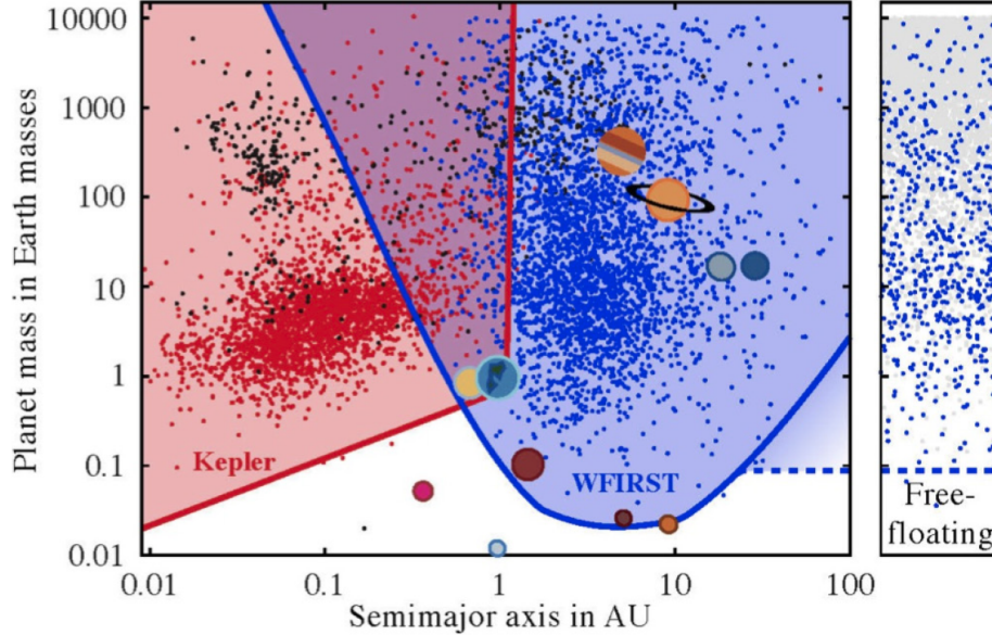
Fig. 3.— The microlensing survey of WFIRST will provide a statistical census for exoplanets with masses down to \sim 0.1 M_{\text{Earth}} and at separations greater than 0.5 au. WFIRST will also be able to probe the population of unbound planets. Source: WFIRST Mission .
