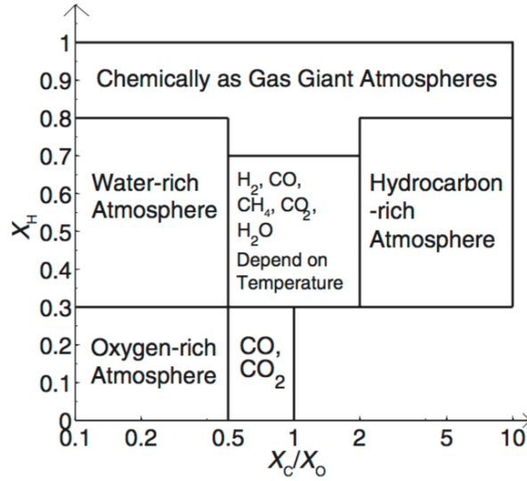
Fig. 17.— The types of thick atmospheres possible on Super-Earths and mini Neptunes, based on the extensive exploration of chemical reaction networks. For atmospheres not dominated by H_2 , different atmosphere classes emerge as a function of the relative abundances of C, O, and H. From Hu & Seager (2014).
