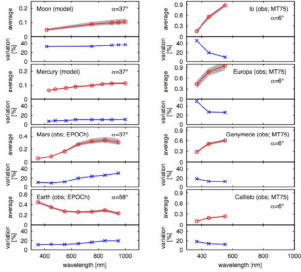
Fig. 12.— Albedo and its variations as a function of wavelengths for Solar System bodies with minor or no atmosphere. From Fujii et al. (2014).
