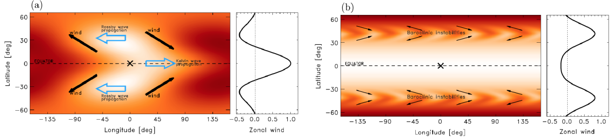
Fig. 20.— Dependence of the atmospheric circulation on rotation rate. Panel (a) shows a slowly-rotating, highly irradiated hot-Jupiter planet with strong day-night temperature difference and a strong eastward equatorial super-rotating jet. Panel (b) shows rapidly rotating warm Jupiters that are weakly irradiated. These planets develop eddy driven zonal jets that peak at mid-latitudes rather than at the equator. From Showman et al. (2015) .
