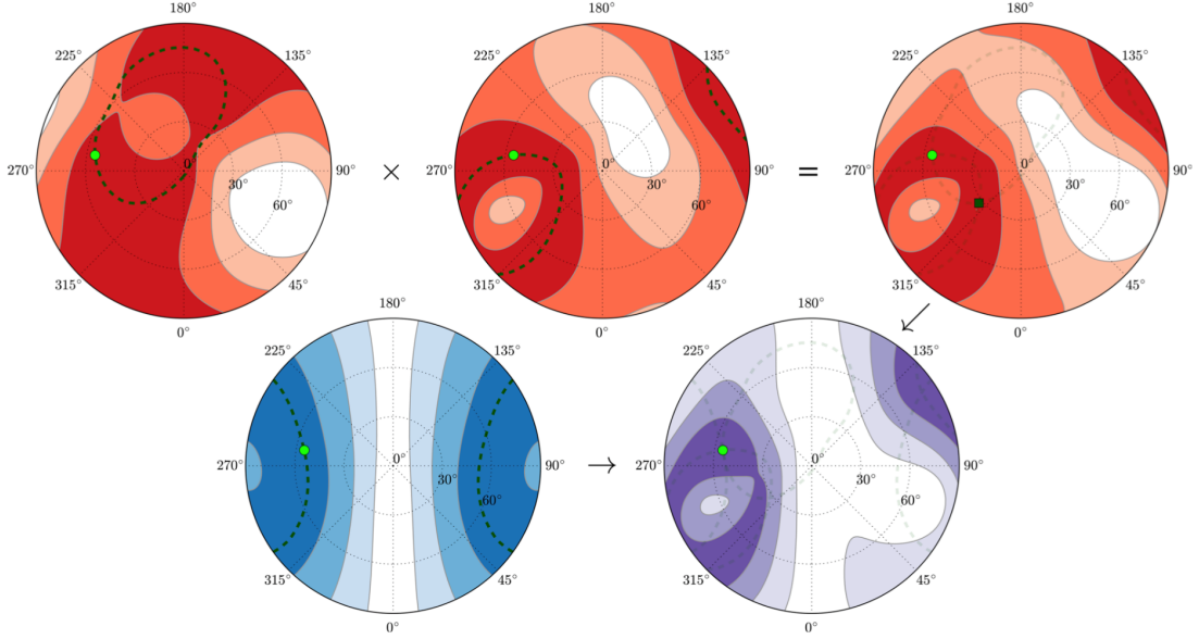
Fig. 11.— Predicted confidence regions for planet’s spin axis, from hypothetical single-and dual-epoch observations. Observing a planet at just a few orbital phases can significantly constrain both its obliquity and axial orientation. Obliquity is plotted radially: the centre is = 0^\circ and the edge is = 90^\circ . The azimuthal angle represents the planets solstice phase. The green circles are the true planet spin axis, while the dark dashed lines and square show idealized constraints assuming perfect knowledge of the orbital geometry and kernel (i.e. no uncertainties). The upper left-hand and centre panels describe planet Q at phase angles 120^\circ and 240^\circ , respectively, while the lower left-hand panel incorporates both phases. For the colored regions, 10^\circ uncertainty is assumed on each kernel width, inclination, and orbital phase, while 20^\circ uncertainty is assumed on the change in dominant colatitude. Regions up to 3\sigma are shown, where darker bands are more likely. From Schwartz et al. (2016) .
