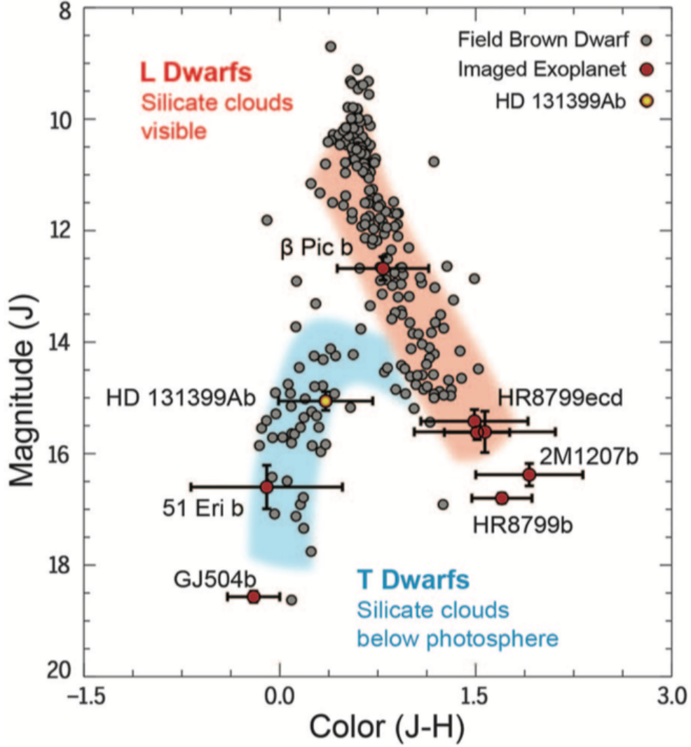
Fig. 14.— Condensate clouds have a fundamental impact on the positions of brown dwarfs and directly imaged exoplanets on the near-infrared color-magnitude diagram. Along the L-type sequence (red) silicate clouds in the upper atmosphere become thicker. The cooler T-dwarfs are bluer because the silicate clouds are below the visible upper atmosphere. Figure from Wagner et al. (2016) , which is in part based on the parallax database by Dupuy & Liu (2012) .
