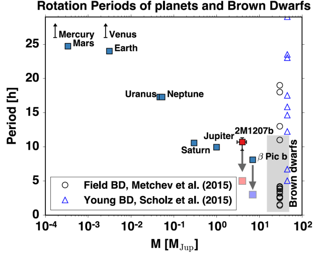
Fig. 8.— Rotation periods provide insights into the properties and formation of planets. A comparison of Solar System planets, directly imaged exoplanets, and brown dwarfs reveals a characteristic mass-dependent rotation rate for massive planets. The ages of the Solar System planets is 4.56 Gyr; the ages of the directly imaged planets is <30 Myr; the ages of the brown dwarfs are few Myr (triangles) and a broad age range for the field objects (triangles). The arrows shows the expected spin-up due to gravitational contraction. From Zhou et al. (2016).
