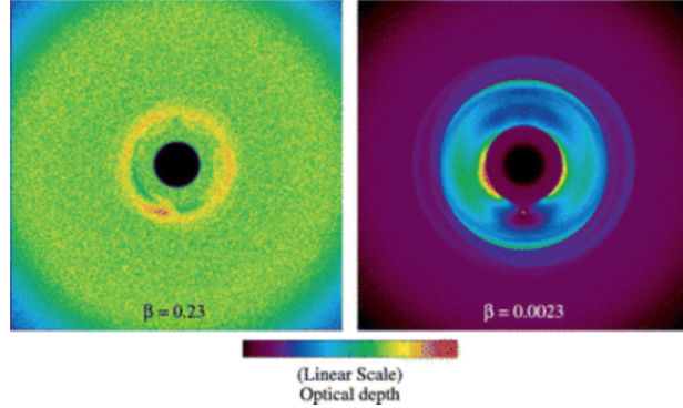
Fig. 6.— Comparison of the optical depths predicted by disk-planet interactions models for a composite cloud formed for a 2 earth-mass planet at 6 au (from Stark & Kuchner 2008). The planet, marked with a white dot, orbits counterclockwise in these images. Left : Optical depth of the smallest particles included in the composite clouds. Right : Optical depth of the largest particles included in the composite clouds. The largest particles dominate the optical depth in a cloud of particles released with a Dohnanyi crushing law, because they are longer-lived and more likely to be trapped in mean motion resonances than smaller particles.
