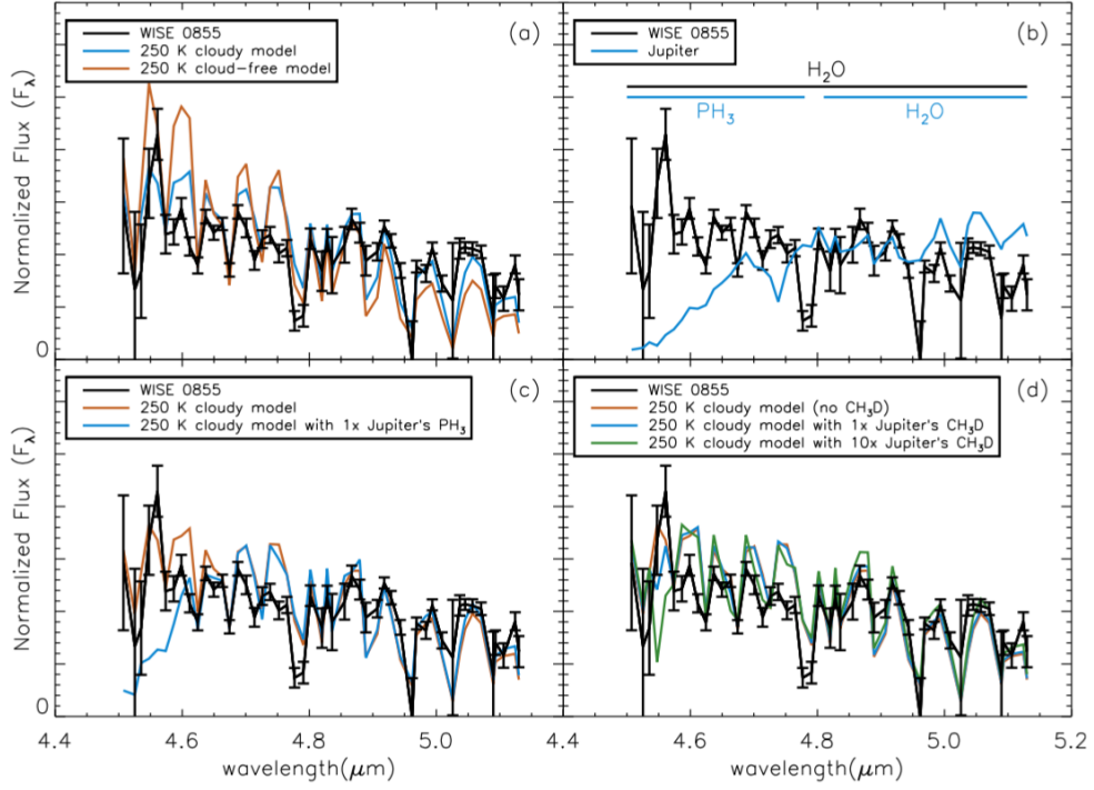
Fig. 15.— Gemini/GNIRS spectrum of the \sim 250 K Y-dwarfs WISE0855 shows a series of absorption features attributable to water vapor, muted by clouds (likely water ice). From Skemer et al. (2016) .
