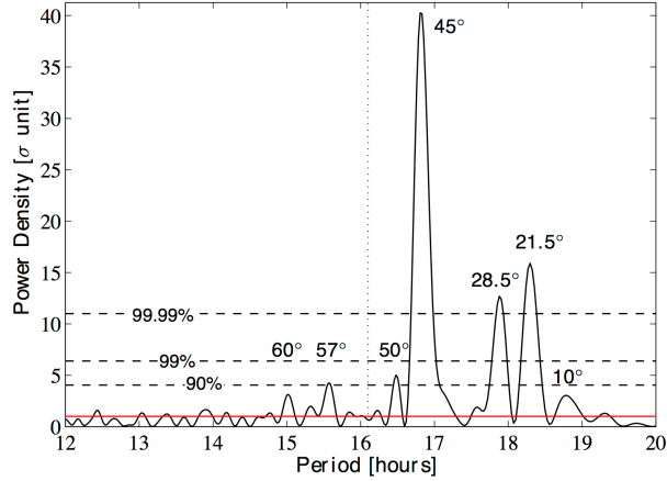
Fig. 7.— Whitened power spectrum from 50-day-long Kepler monitoring of hemisphere-integrated reflected light Neptune, with the most significant peak corresponding to the rotation period. Numbers above some peaks indicate the latitudes on Neptune corresponding to that rotation period based on the zonal velocities. From Simon et al. (2016).
