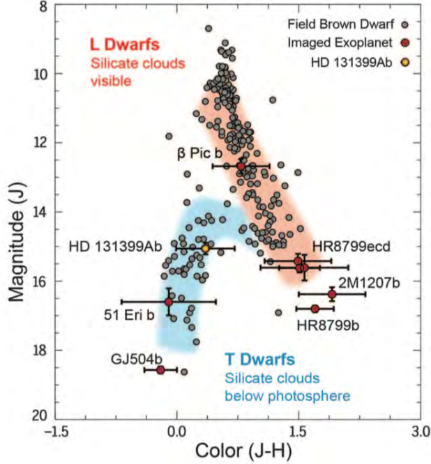
Fig. 14.— Condensate clouds have a fundamental impact on the positions of brown dwarfs and directly imaged exoplanets on the near-infrared color-magnitude diagram. Along the L-type sequence (red) silicate clouds in the upper atmosphere become thicker. The cooler T-dwarfs are bluer because the silicate clouds are below the visible upper atmosphere. Figure from Wagner et al. (2016) , which is in part based on the parallax database by Dupuy & Liu (2012) .
