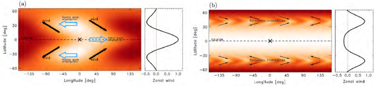
Fig. 20.— Dependence of the atmospheric circulation on rotation rate. Panel (a) shows a slowly-rotating, highly irradiated hot-Jupiter planet with strong day-night temperature difference and a strong eastward equatorial super-rotating jet. Panel (b) shows rapidly rotating warm Jupiters that are weakly irradiated. These planets develop eddy driven zonal jets that peak at mid-latitudes rather than at the equator. From Showman et al. (2015) .
