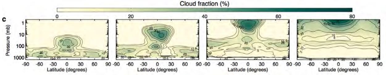
Fig. 21.— Moist/water-rich atmosphere simulations from (Wolf & Toon 2015). The four panels indicate the amount of cloud water content on a planet at different insolation levels (or, alternately, how close to an inner edge of the HZ a planet is located). From left to right, the solar insolation varies: S_0 (current Earth insolation), 110% of S_0 , 112.5% S_0 and 121% of S_0 . This is for an Earth-size planet around a Sun-like star.
