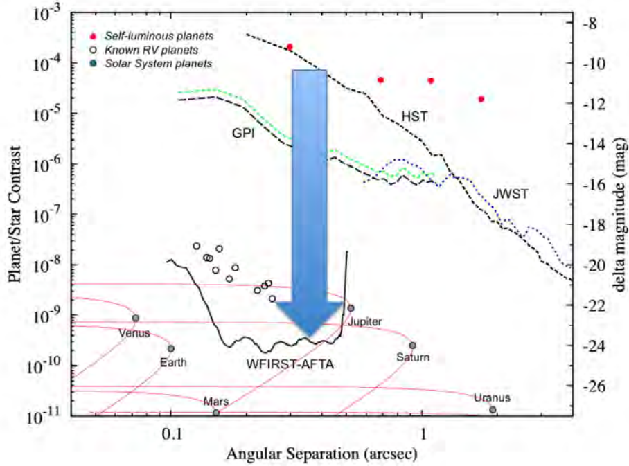
Fig. 4.— The goal of the WFIRST’s coronagraphic instrument is to image giant exoplanets and disks at 5 au and greater separations. The sample of planets that WFIRST will be able to image include known radial velocity planets. Source: WFIRST Mission .
