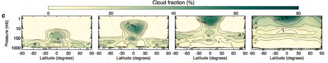
Fig. 20.— Moist/water-rich atmosphere simulations from (Wolf & Toon 2015). The four panels indicate the amount of cloud water content on a planet at different insolation levels (or, alternately, how close to an inner edge of the HZ a planet is located). From left to right, the solar insolation varies: S_0 (current Earth insolation), 110% of S_0 , 112.5% S_0 and 121% of S_0 . This is for an Earth-size planet around a Sun-like star.
