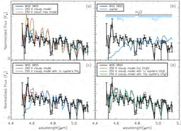
Fig. 14.— Gemini/GNIRS spectrum of the \sim 250 K Y-dwarfs WISE0855 shows a series of absorption features attributable to water vapor, muted by clouds (likely water ice). From Skemer et al. (2016) .
