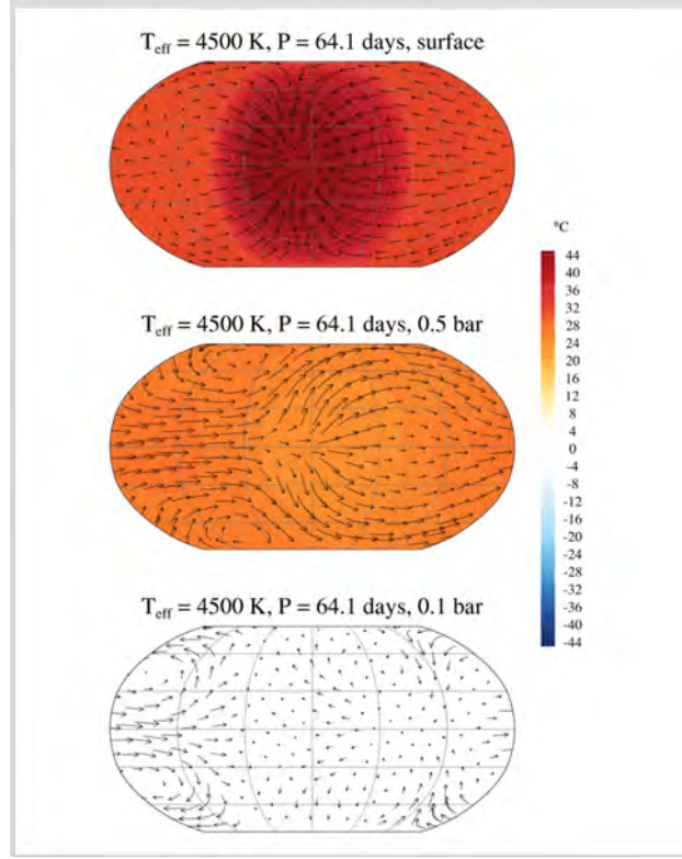
Fig. 21.— Temperature and horizontal wind vectors at the surface, 0.5 bar, and 0.1 bar levels for an Earth-mass planet in a slow-rotating regime near the inner edge of the habitable zone around a K-dwarf. Slowly rotating planets develop sub-stellar clouds that increase the albedo of the planet. Inflow along the equator and from the poles into the substellar point at the center is also shown. From Kopparapu et al. (2016) .
