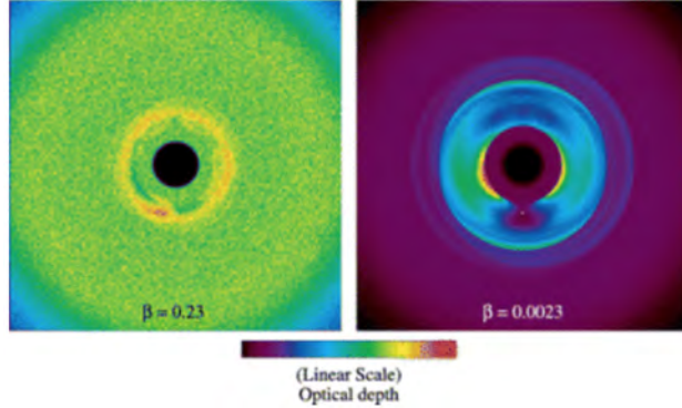
Fig. 5.— Comparison of the optical depths predicted by disk-planet interactions models for a composite cloud formed for a 2 earth-mass planet at 6 au (from Stark & Kuchner 2008 ). The planet, marked with a white dot, orbits counterclockwise in these images. Left : Optical depth of the smallest particles included in the composite clouds. Right : Optical depth of the largest particles included in the composite clouds. The largest particles dominate the optical depth in a cloud of particles released with a Dohnanyi crushing law, because they are longer-lived and more likely to be trapped in mean motion resonances than smaller particles.
