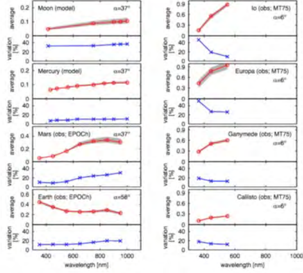
Fig. 11.— Albedo and its variations as a function of wavelengths for Solar System bodies with minor or no atmosphere. From Fujii et al. (2014).
