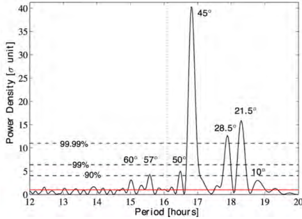
Fig. 6.— Whitened power spectrum from 50-day-long Kepler monitoring of hemisphere-integrated reflected light Neptune, with the most significant peak corresponding to the rotation period. Numbers above some peaks indicate the latitudes on Neptune corresponding to that rotation period based on the zonal velocities. From Simon et al. (2016).
