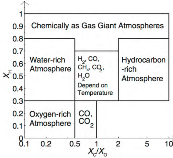
Fig. 16.— The types of thick atmospheres possible on Super-Earths and mini Neptunes, based on the extensive exploration of chemical reaction networks. For atmospheres not dominated by H_2 , different atmosphere classes emerge as a function of the relative abundances of C, O, and H. From Hu & Seager (2014) .
