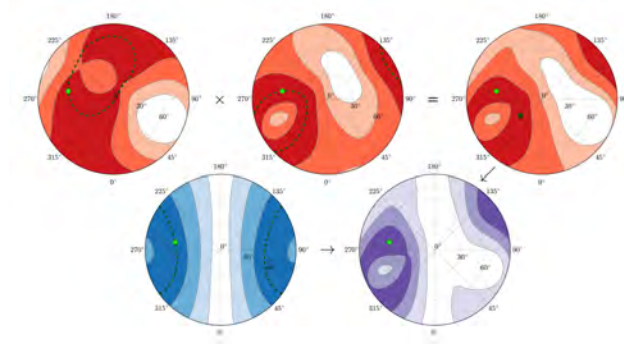
Fig. 10.— Predicted confidence regions for planet’s spin axis, from hypothetical single- and dual-epoch observations. Observing a planet at just a few orbital phases can significantly constrain both its obliquity and axial orientation. Obliquity is plotted radially: the centre is = 0^\circ and the edge is = 90^\circ . The azimuthal angle represents the planet’s solstice phase. The green circles are the true planet spin axis, while the dark dashed lines and square show idealized constraints assuming perfect knowledge of the orbital geometry and kernel (i.e. no uncertainties). The upper left-hand and centre panels describe planet Q at phase angles 120^\circ and 240^\circ , respectively, while the lower left-hand panel incorporates both phases. For the colored regions, 10^\circ uncertainty is assumed on each kernel width, inclination, and orbital phase, while 20^\circ uncertainty is assumed on the change in dominant colatitude. Regions up to 3\sigma are shown, where darker bands are more likely. From Schwartz et al. (2016) .
