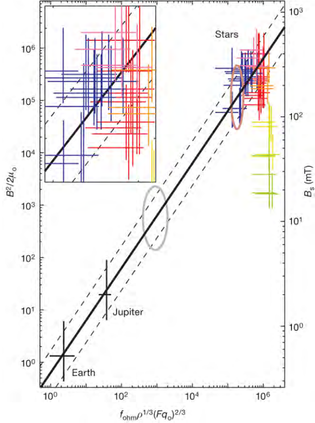
Fig. 8.— The comparison between Earth, Jupiter, and stars shows that the magnetic energy density (in the dynamo) strongly correlates with a function of density and bolometric flux (here both in units of \text{J m}^{-3} ). The bar lengths show estimated uncertainty rather than formal error. The stellar field is enlarged in the inset. Brown and grey ellipses indicate predicted locations of a brown dwarf with 1,500 K surface temperature and an extrasolar planet with seven Jupiter masses, respectively. From Christensen et al. (2009) .
