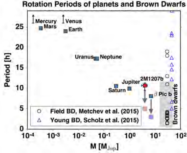
Fig. 7.— Rotation periods provide insights into the properties and formation of planets. A comparison of Solar System planets, directly imaged exoplanets, and brown dwarfs reveals a characteristic mass-dependent rotation rate for massive planets. The ages of the Solar System planets is 4.56 Gyr; the ages of the directly imaged planets is <30 Myr; the ages of the brown dwarfs are few Myr (triangles) and a broad age range for the field objects (triangles). The arrows shows the expected spin-up due to gravitational contraction. From Zhou et al. (2016).
