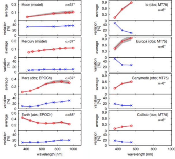
Fig. 7.— Albedo and its variations as a function of wavelengths for Solar System bodies with minor or no atmosphere. From Fujii et al. (2014).
