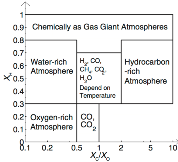
Fig. 11.— The types of thick atmospheres possible on Super-Earths and mini Neptunes, based on the extensive exploration of chemical reaction networks. For atmospheres not dominated by H 2 , different atmosphere classes emerge as a function of the relative abundances of C, O, and H. From Hu & Seager (2014).
