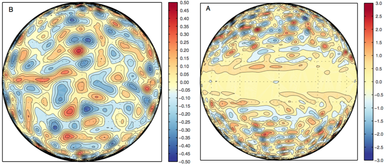
Fig. 12.— Depending on the relative importance of rotational speed, wind speed, and vertical heat transport, simple models predict two different regimes of circulation for giant planets: vortex-dominated (left) and jet-dominated (right). From Zhang & Showman (2014).
