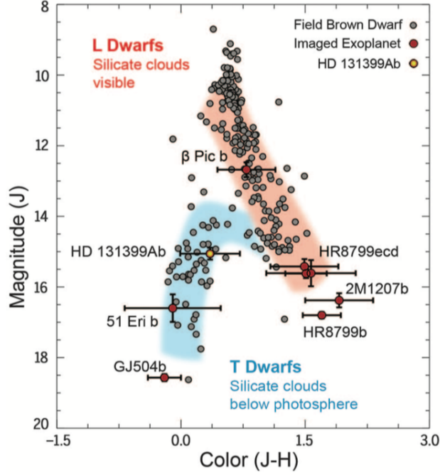
Fig. 9.— Condensate clouds have a fundamental impact on the positions of brown dwarfs and directly imaged exoplanets on the near-infrared color-magnitude diagram. Along the L-type sequence (red) silicate clouds in the upper atmosphere become thicker. The cooler T-dwarfs are bluer because the silicate clouds are below the visible upper atmosphere. Figure from Wagner et al. (2016), which is in part based on the parallax database by Dupuy & Liu (2012).
