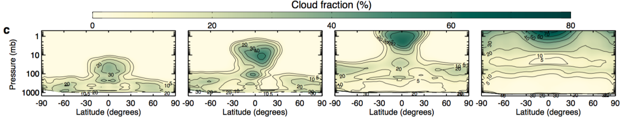
Fig. 14.— Moist/water-rich atmosphere simulations from (Wolf & Toon 2015). The four panels indicate the amount of cloud water content on a planet at different insolation levels (or, alternately, how close to an inner edge of the HZ a planet is located). From left to right, the solar insolation varies: S_0 (current Earth insolation), 10% of S_0 , 12.5% S_0 and 21% of S_0 . This is for an Earth-size planet around a Sun-like star.
