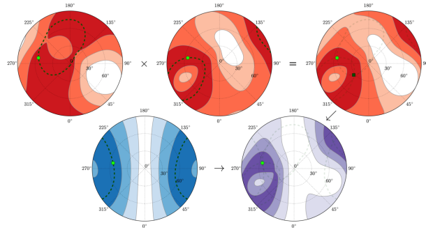
Fig. 6.— Predicted confidence regions for planet’s spin axis, from hypothetical single- and dual-epoch observations. Observing a planet at just a few orbital phases can significantly constrain both its obliquity and axial orientation. Obliquity is plotted radially: the centre is = 0^\circ and the edge is = 90^\circ . The azimuthal angle represents the planet’s solstice phase. The green circles are the true planet spin axis, while the dark dashed lines and square show idealized constraints assuming perfect knowledge of the orbital geometry and kernel (i.e. no uncertainties). The upper left-hand and centre panels describe planet Q at phase angles 120^\circ and 240^\circ , respectively, while the lower left-hand panel incorporates both phases. For the colored regions, 10^\circ uncertainty is assumed on each kernel width, inclination, and orbital phase, while 20^\circ uncertainty is assumed on the change in dominant colatitude. Regions up to 3\sigma are shown, where darker bands are more likely. From Schwartz et al. (2016).
