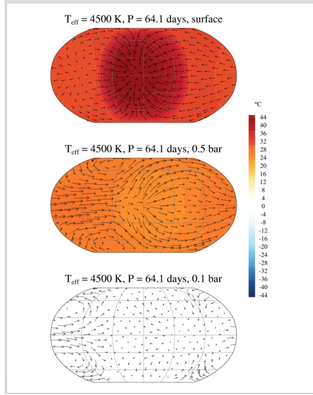
Fig. 15.— Temperature and horizontal wind vectors at the surface, 0.5 bar, and 0.1 bar levels for an Earth-mass planet in a slow-rotating regime near the inner edge of the habitable zone around a K-dwarf. Slowly rotating planets develop sub-stellar clouds that increase the albedo of the planet. Inflow along the equator and from the poles into the substellar point at the center is also shown. From Kopparapu et al. (2016).
