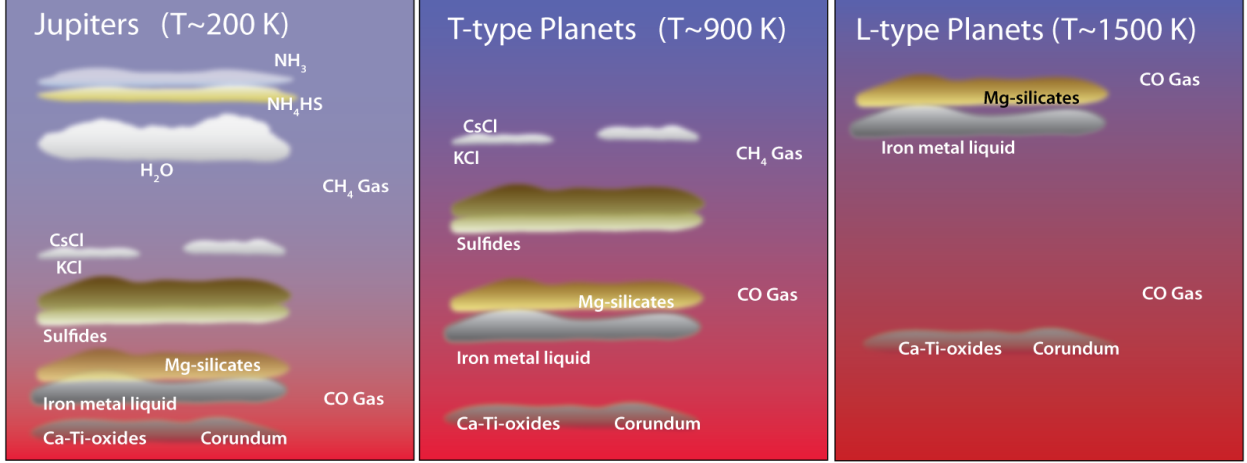
Fig. 8.— Condensate clouds predicted for the upper atmospheres of giant planets of different temperature. By D. Apai, after Lodders (2003).
