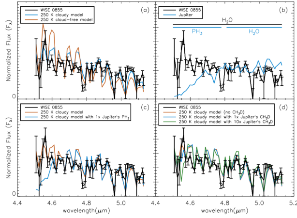
Fig. 10.— Gemini/GNIRS spectrum of the \sim 250 K Y-dwarfs WISE0855 shows a series of absorption features attributable to water vapor, muted by clouds (likely water ice). From Skemer et al. (2016).
