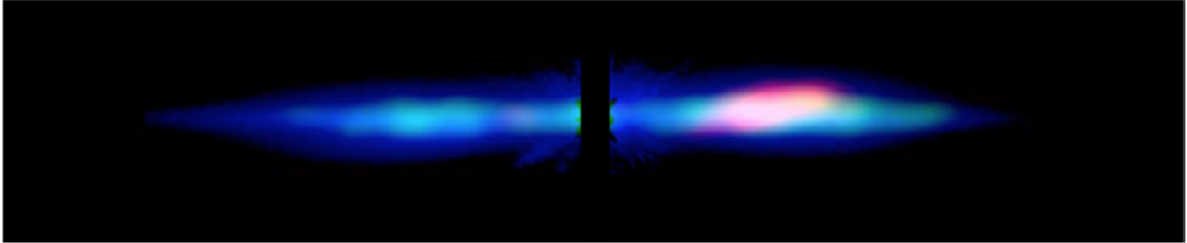
Figure 14. Key structures in the \beta Pic system, as derived from multi-wavelength imaging.
