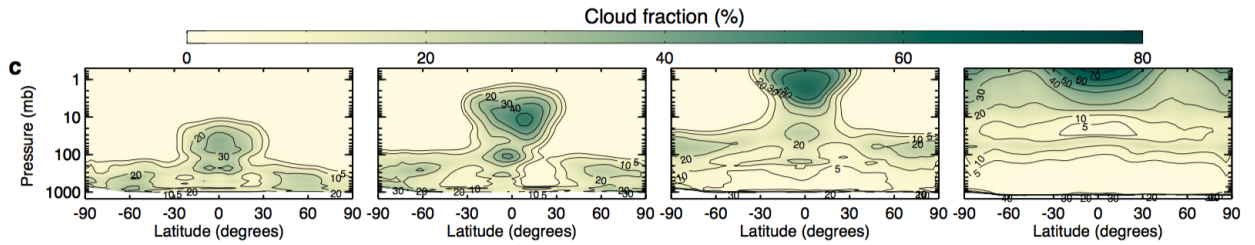
Fig. 9.— Moist/water-rich atmosphere simulations from Wolf & Toon(2015). The four panels indicate the amount of cloud fraction on a planet at different insulations (or alternately how close to an inner edge of the HZ a planet is located). From left to right, the solar insolation varies S_0 (current Earth insolation), 10% of S_0 , 12.5% S_0 and 21% of S_0 . This is for an Earth-size planet around a Sun-like star.
