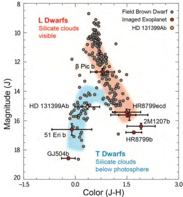
Fig. 10.— Condensate clouds have a fundamental impact on the positions of brown dwarfs and directly imaged exoplanets on the near-infrared color-magnitude diagram. Along the L-type sequence (red) silicate clouds in the upper atmosphere become thicker. The cooler T-dwarfs are bluer because the silicate clouds are below the visible upper atmosphere. Figure from Wagner et al. (2016), which is in part based on the parallax database by Dupuy & Liu (2012).
