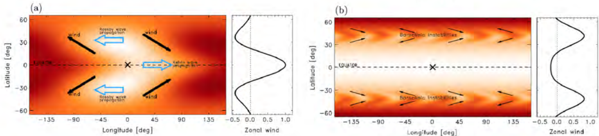
Fig. 16.— Dependence of the atmospheric circulation on rotation rate. Panel (a) shows a slowly-rotating, highly irradiated hot-Jupiter planet with strong day-night temperature difference and a strong eastward equatorial super-rotating jet. Panel (b) shows rapidly rotating warm Jupiters that are weakly irradiated. These planets develop eddy driven zonal jets that peak at mid-latitudes rather than at the equator. From Showman et al. (2015).
