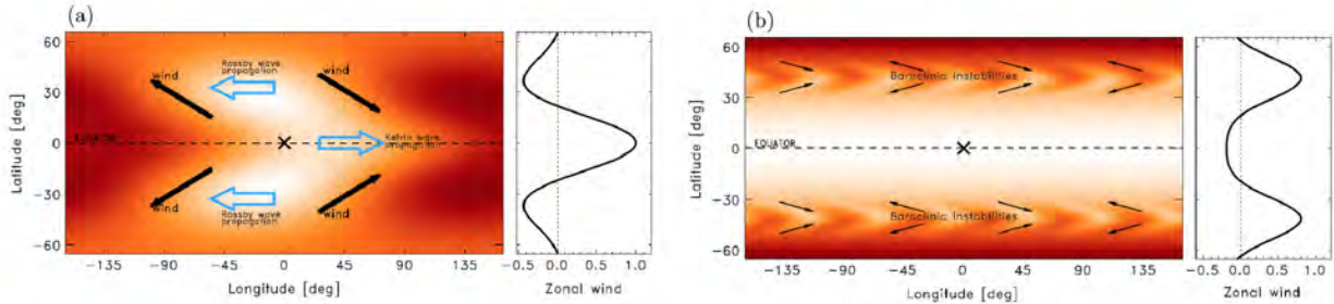
Fig. 15.— Dependence of the atmospheric circulation on rotation rate. Panel (a) shows a slowly-rotating, highly irradiated hot-Jupiter planet with strong day-night temperature difference and a strong eastward equatorial super-rotating jet. Panel (b) shows rapidly rotating warm Jupiters that are weakly irradiated. These planets develop eddy driven zonal jets that peak at mid-latitudes rather than at the equator. From Showman et al. (2015).
