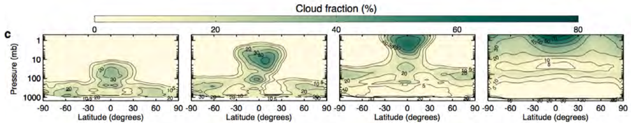
Fig. 16.— Moist/water-rich atmosphere simulations from (Wolf & Toon 2015). The four panels indicate the amount of cloud water content on a planet at different insolation levels (or, alternately, how close to an inner edge of the HZ a planet is located). From left to right, the solar insolation varies: S_0 (current Earth insolation), 110% of S_0 , 112.5% S_0 and 121% of S_0 . This is for an Earth-size planet around a Sun-like star.
