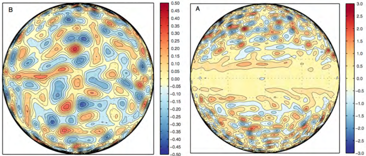
Fig. 14.— Depending on the relative importance of rotational speed, wind speed, and vertical heat transport, simple models predict two different regimes of circulation for giant planets: vortex-dominated (left) and jet-dominated (right). From Zhang & Showman (2014).
