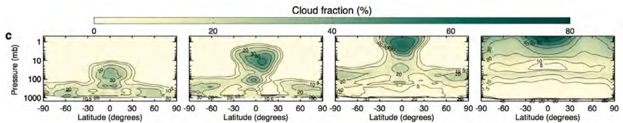
Fig. 11.— Moist/water-rich atmosphere simulations from Wolf & Toon(2014). The four panels indicate the amount of cloud fraction on a planet at different insulations (or alternately how close to an inner edge of the HZ a planet is located). From left to right, the solar insolation varies S_0 (current Earth insolation), 10% of S_0 , 12.5% S_0 and 21% of S_0 . This is for an Earth-size planet around a Sun-like star.
