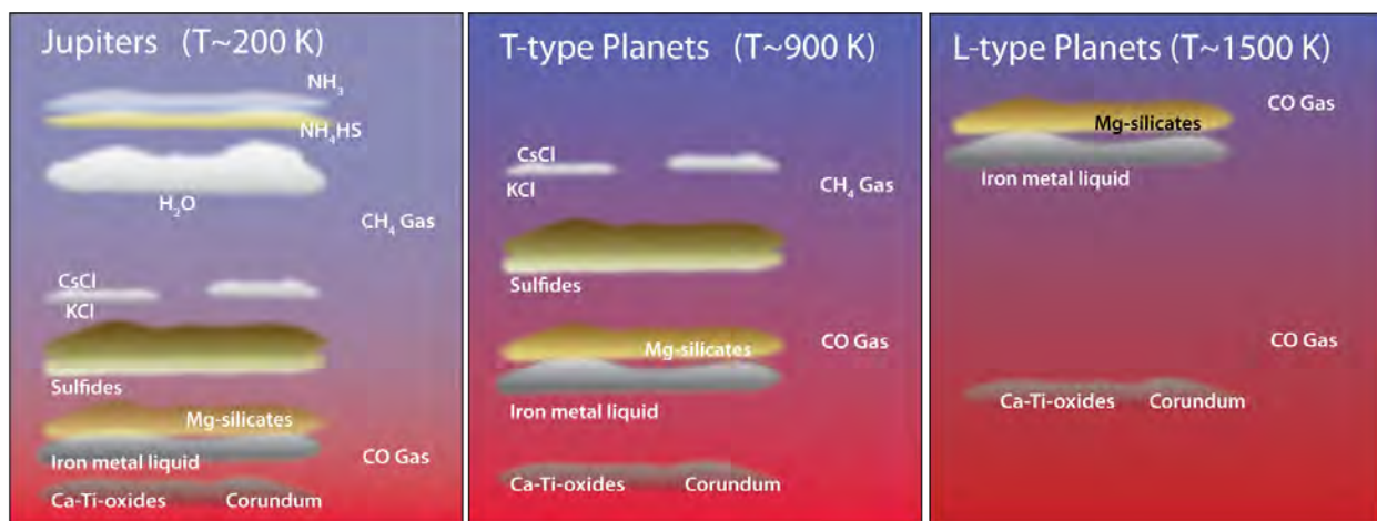
Fig. 7.— Condensate clouds predicted for the upper atmospheres of planets of different temperature. By D. Apai, after Lodders (2003).
