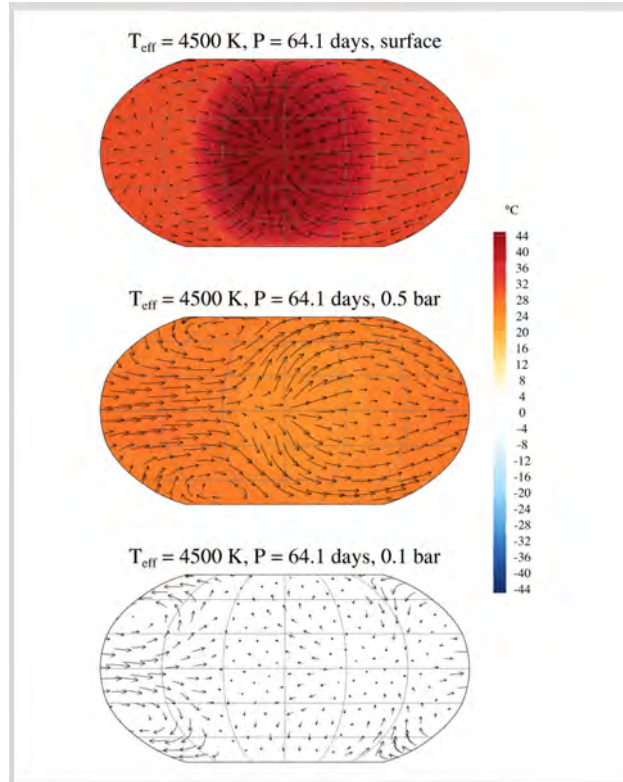
Fig. 12.— Temperature and horizontal wind vectors at the surface, 0.5 bar, and 0.1 bar levels for an Earth-mass planet in a slow-rotating regime near the inner edge of the habitable zone around a K-dwarf. Slowly rotating planets develop subs-stellar clouds that increase the albedo of the planet. Inflow along the equator and from the poles into the substellar point at the center is also shown. From Kopparapu et al. (2016).
